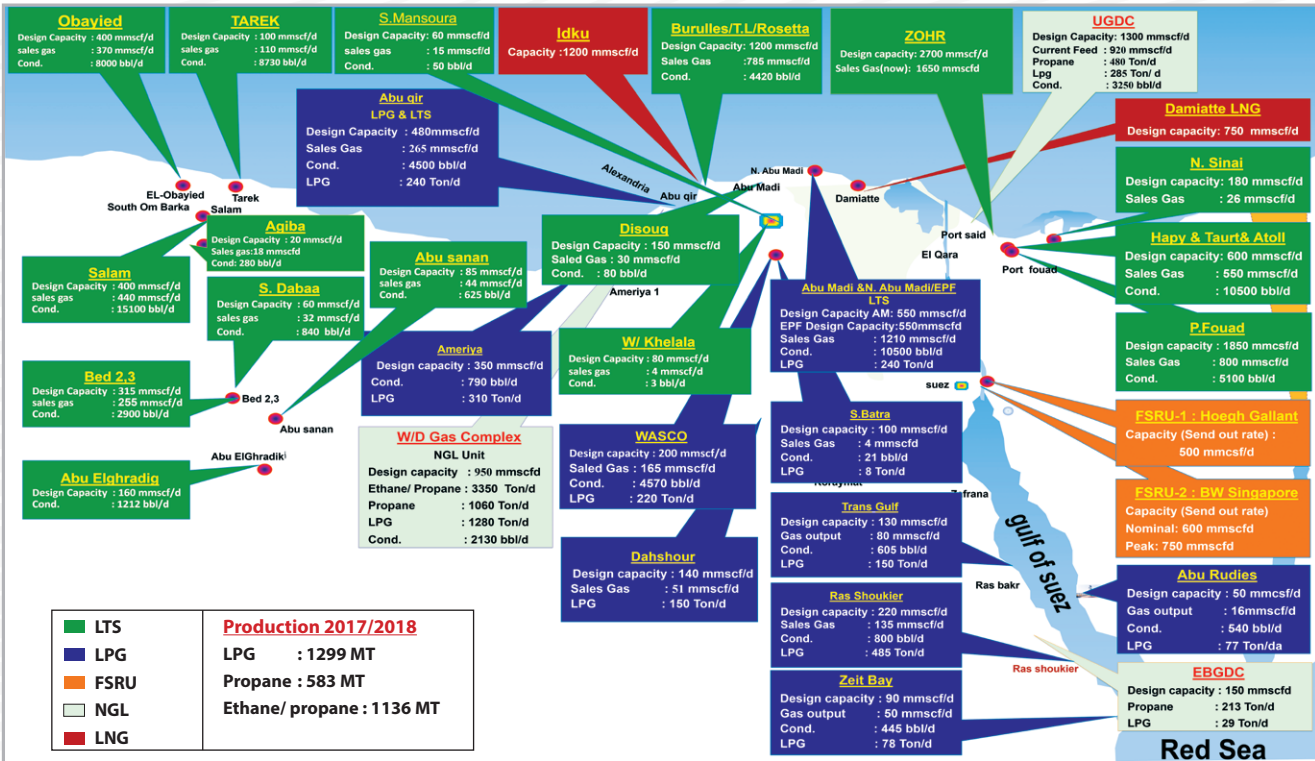
EGYPTIAN GAS FACILITIES
