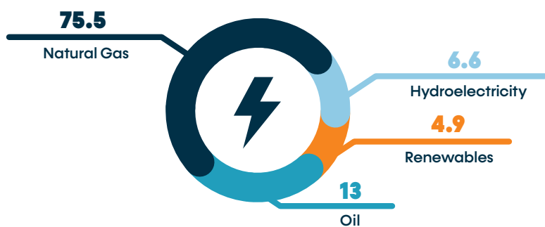
ELECTRICITY GENERATION BREAKDOWN (%)
